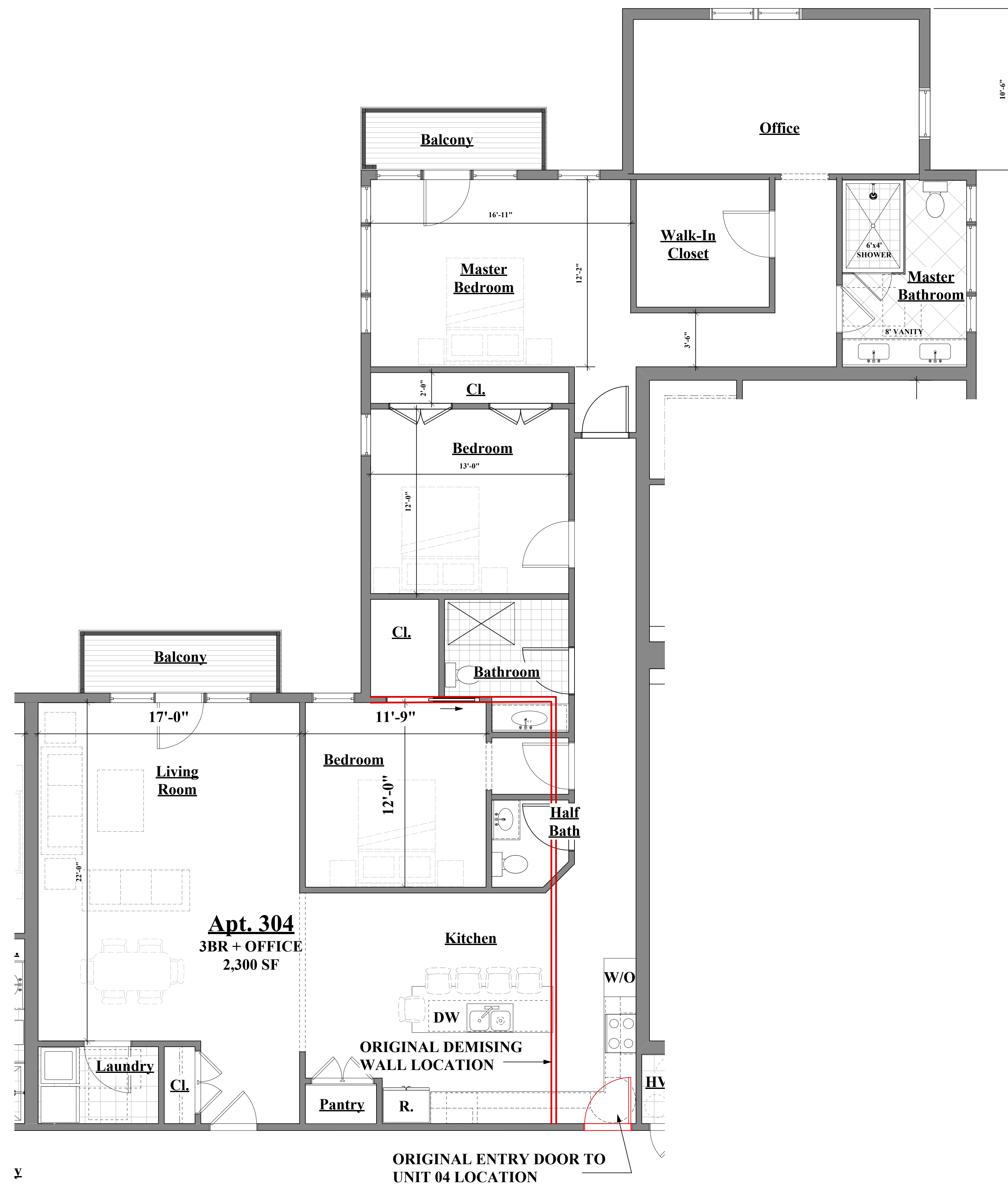
PROPOSED COMBINED UNIT 04 AND 06
